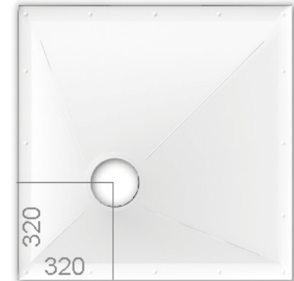
Wetroom Floor Former 1000 x 1000mm - 22mm Depth
